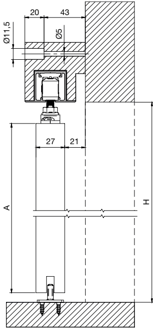
1 Kit SF-P70 READY pletina . 39.0174.9 / 39.0176.0
